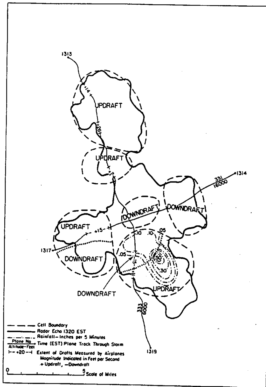
FIG. 16. Radar echo, plane paths, measured draft data, and cell outlines, 1320 EST 9 July 1946.
